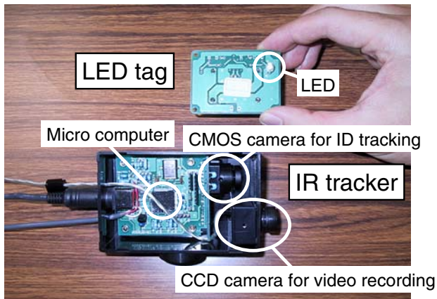
Fig. 3 IR tracker and LED tag
